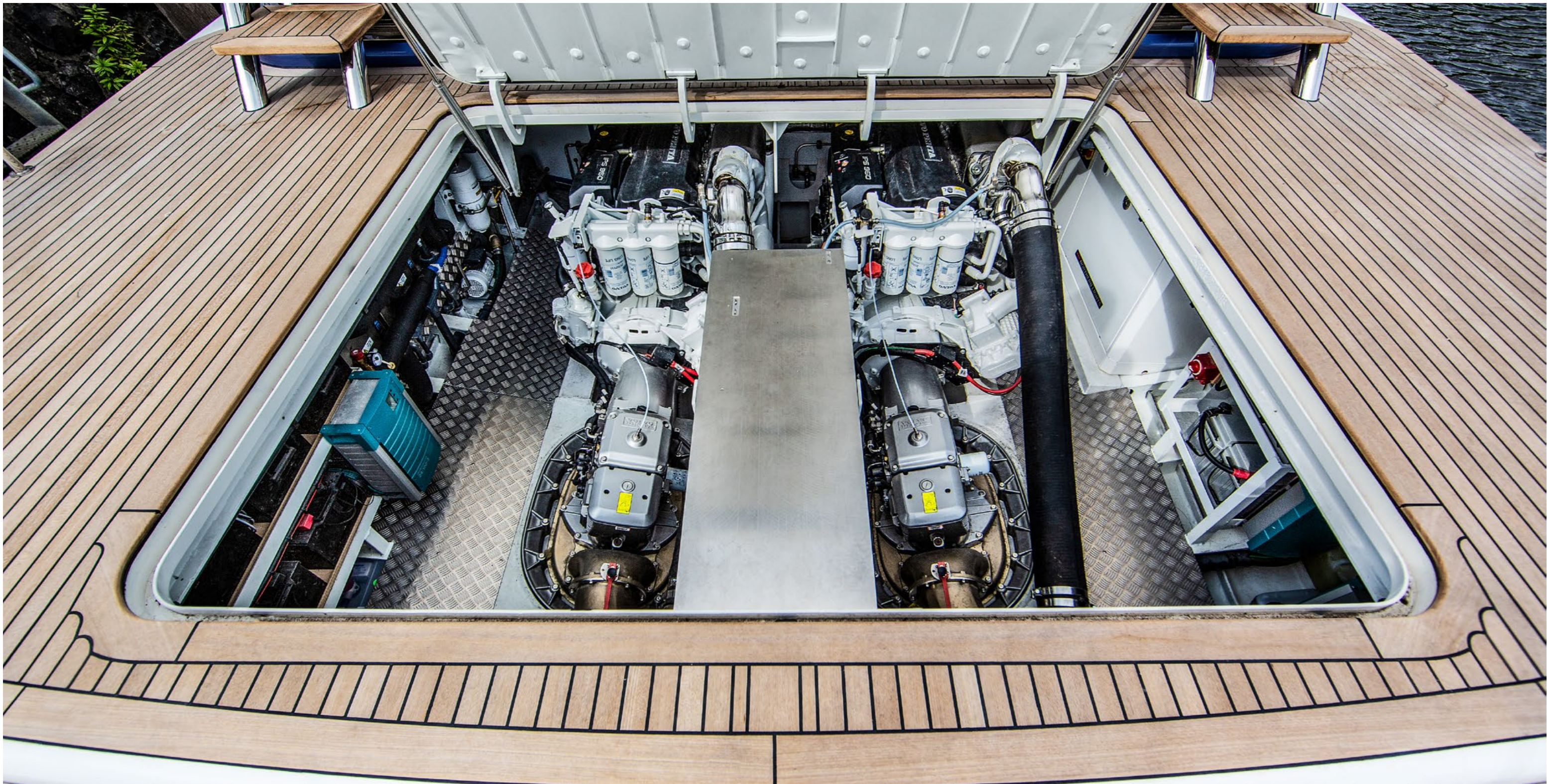
THE ENGINE ROOM IS LOCATED INSIDE THE SWIM PLATFORM
