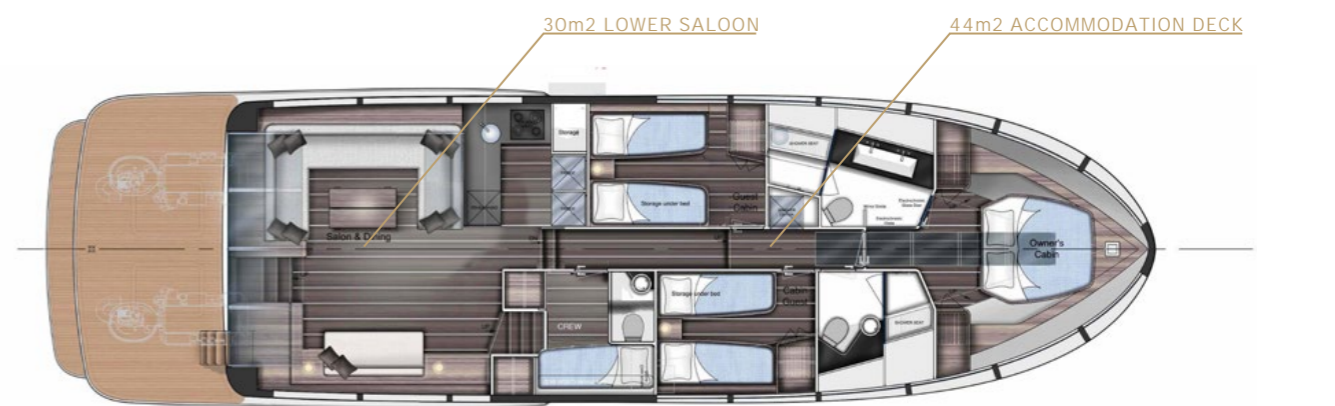
LOWER DECK
