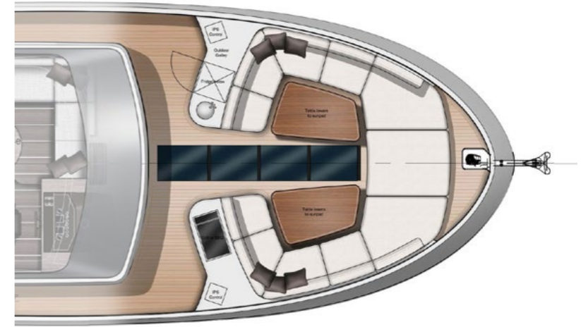
FRONT DECK – OPTION C
